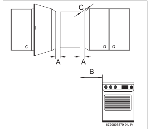
Fig. 5 Minimum distances
