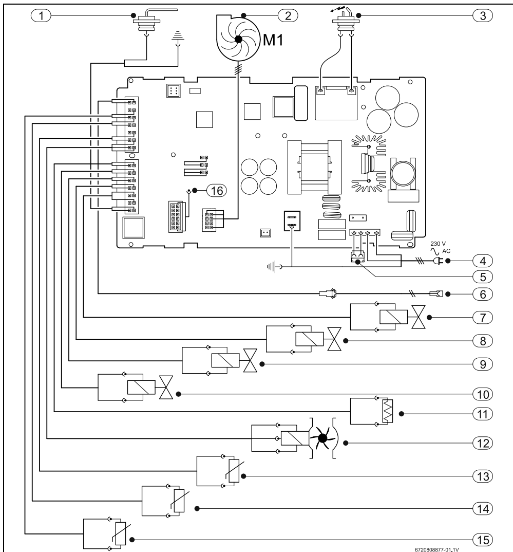
Fig. 3 Electrical diagram
