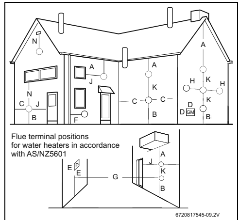
Fig. 6 Minimum flue clearances
